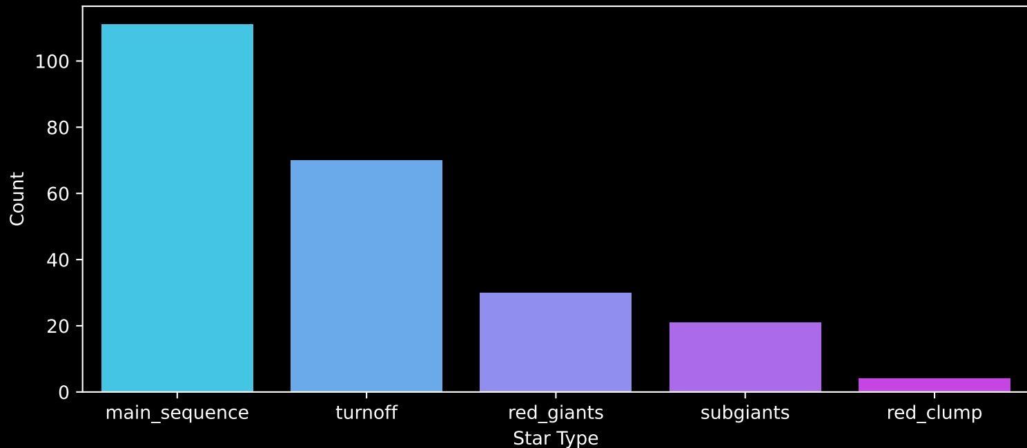
GALAH DR4 Field: [1420] Count plot of Star Type
