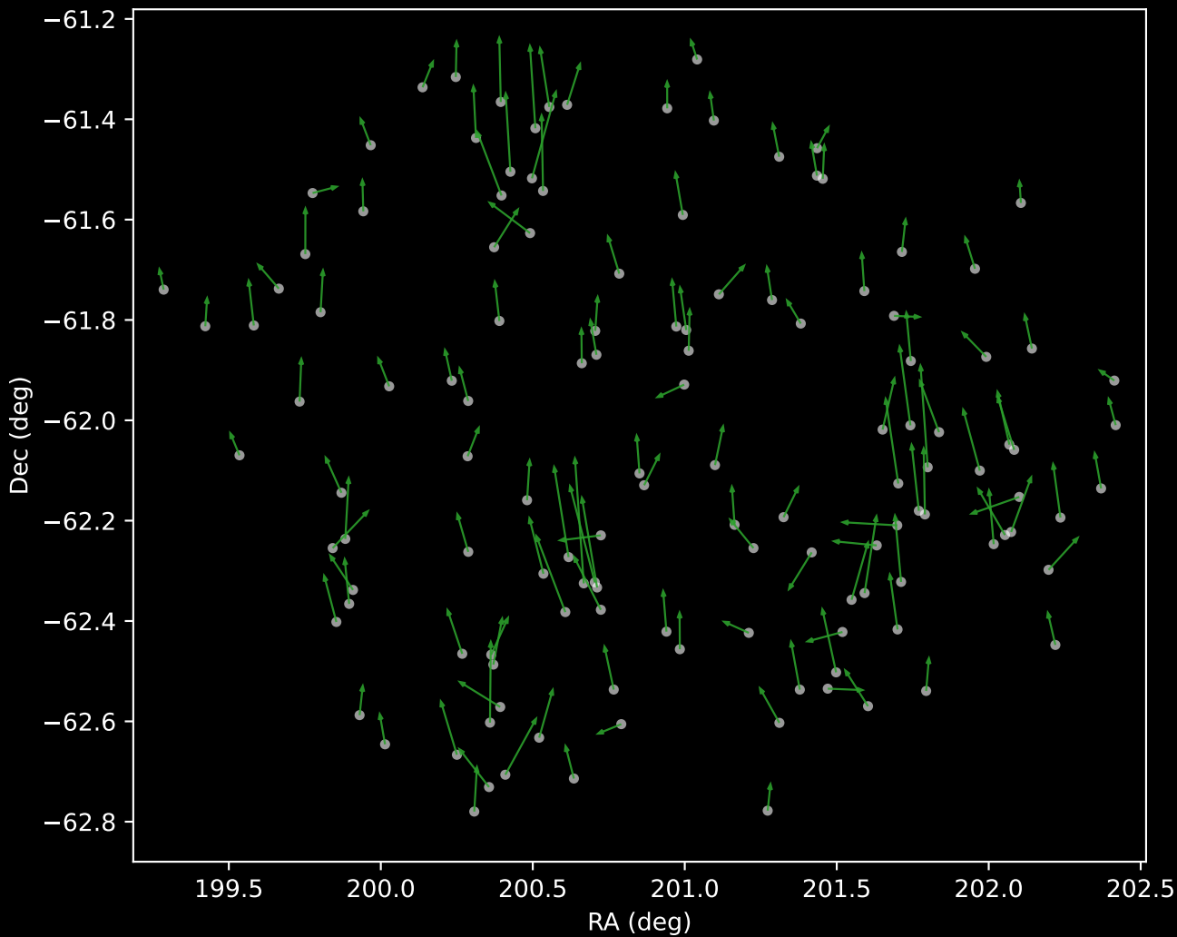
GALAH DR4 Cluster 4 Proper Motion Vectors (n=131)
