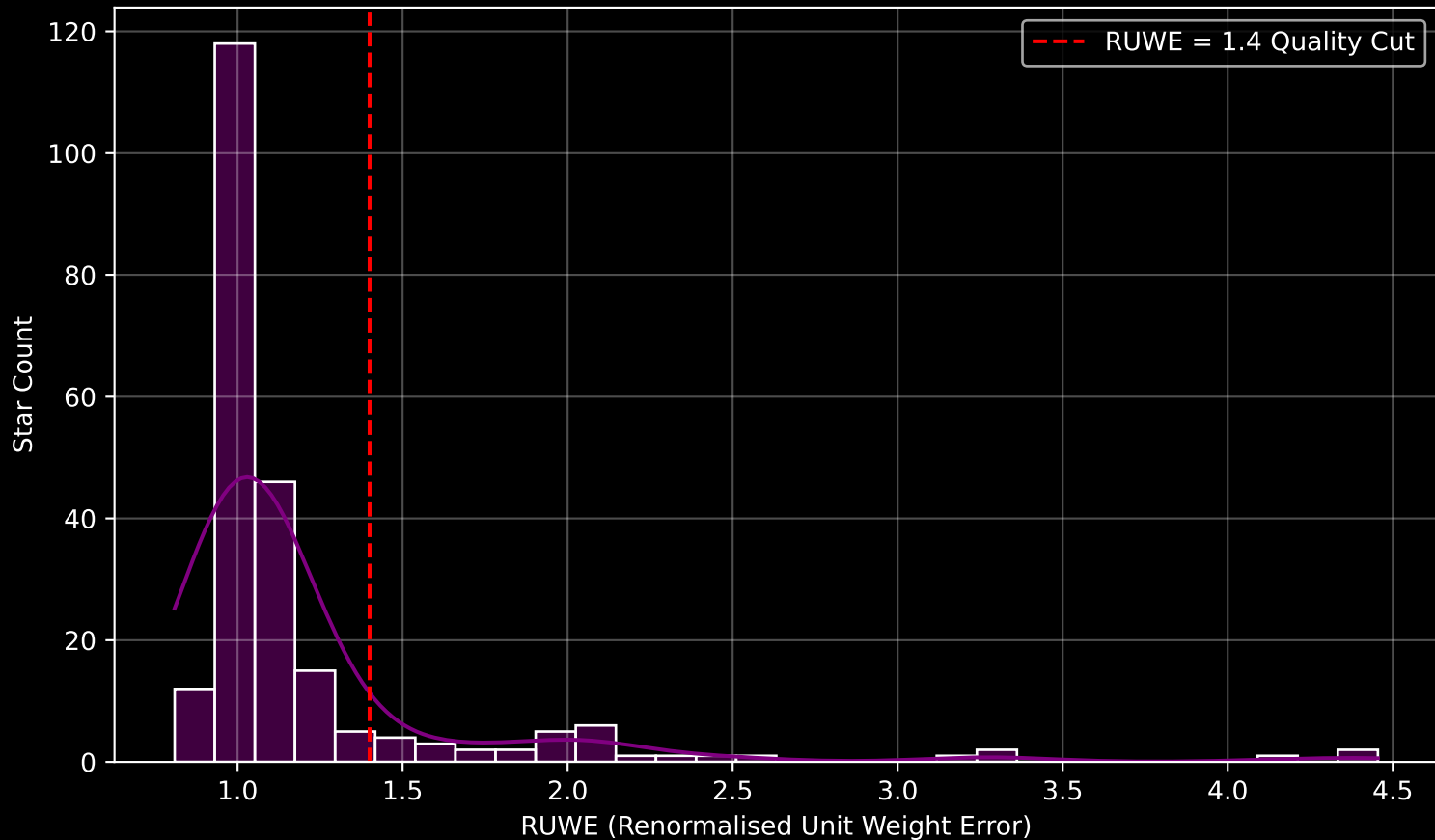
GALAH DR4 Field [1420] RUWE Distribution (n= 228)
